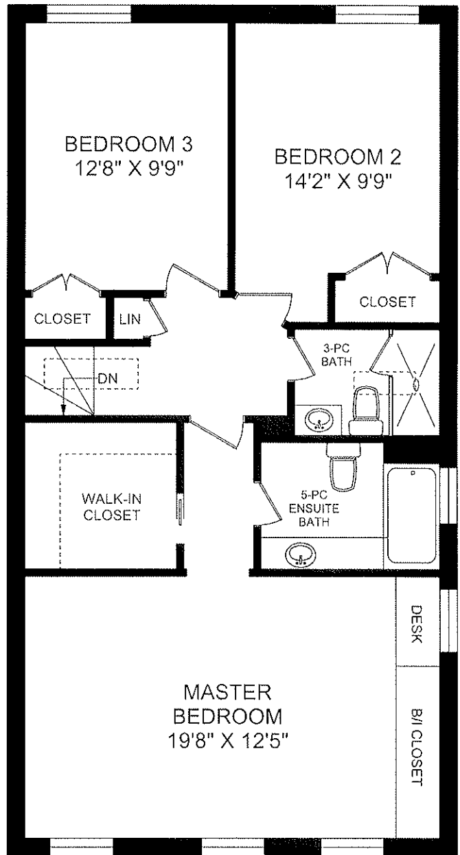
SECOND FLOOR 862 SQUARE FEET
